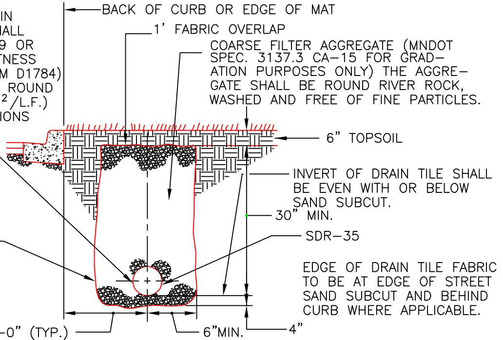
SECTIONAL VIEW
